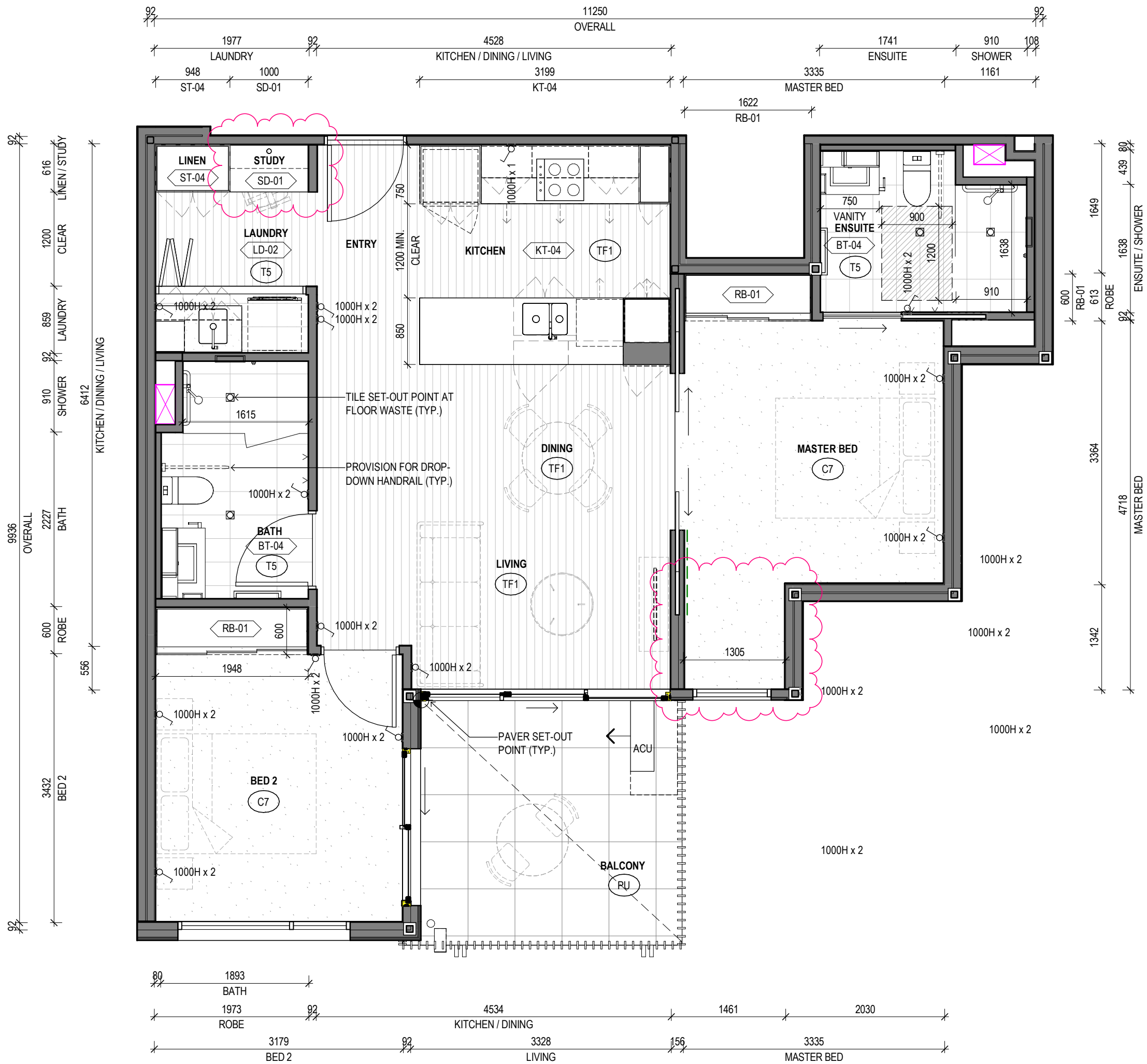
1 ILA Type 12 Scale 1:50
